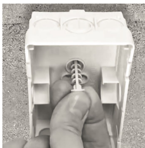
With the DSN 30 you will successfully fasten fire detectors, lamps and sockets at the push of a thumb.
